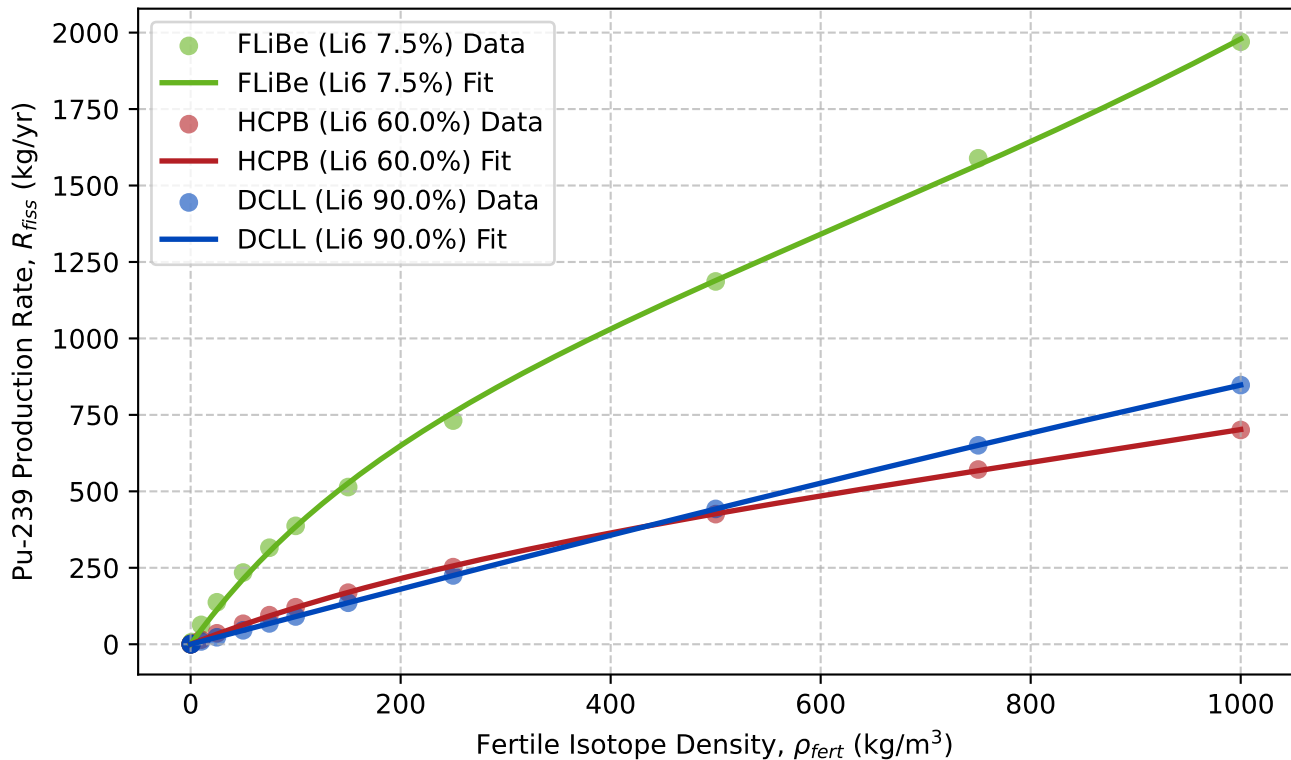
Fissile Production Rate vs. Fertile Density (Blanket Comparison)
